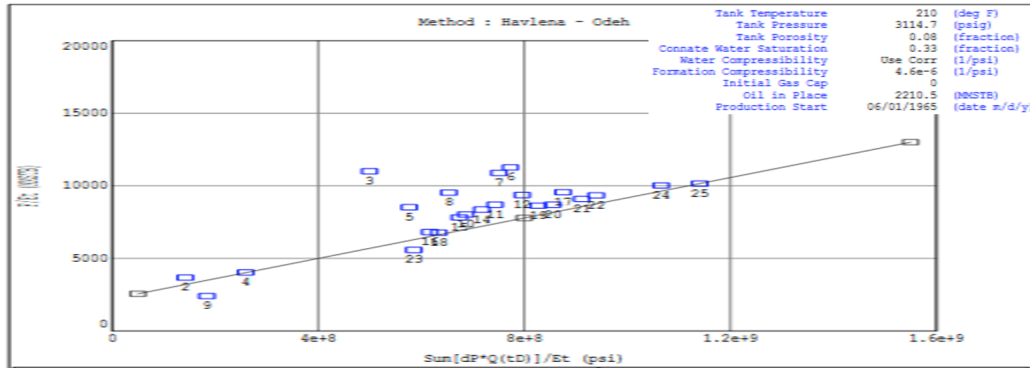
Figure 5: MBAL software result for estimation OOIP by using MBE method, analysis window (7) .
