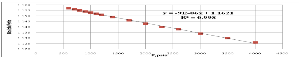
Figure 3: Curve fitting for B_o vs pressure.
