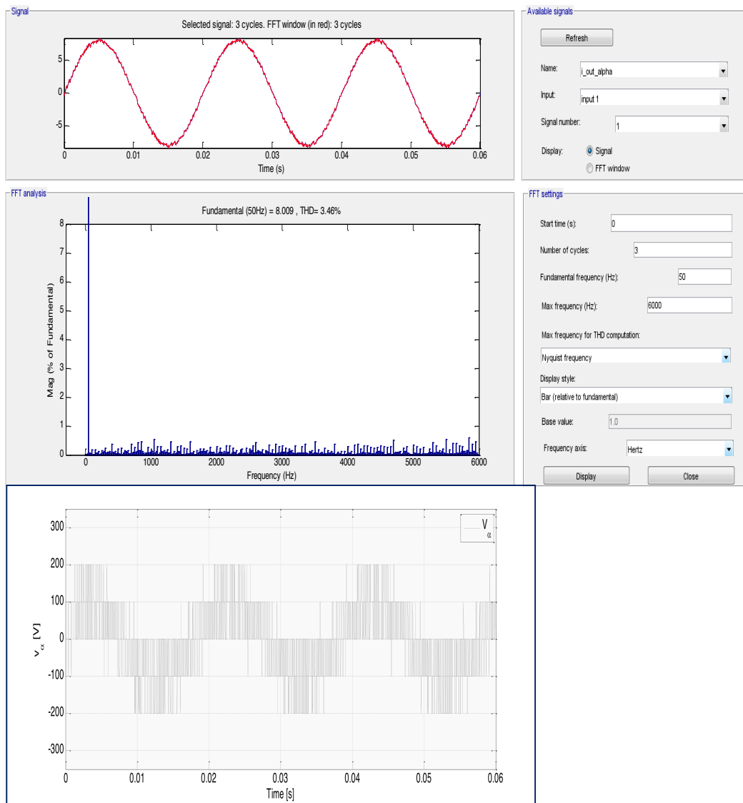
Figure 3: Output current and its magnitude value and output voltage at designed values.
