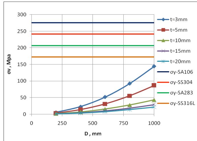
Figure 4: The von-Mises stress ( \sigma_v ) as a function of vessel diameter and thickness.
