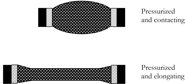
Figure 1: Concept of McKibben actuator.
