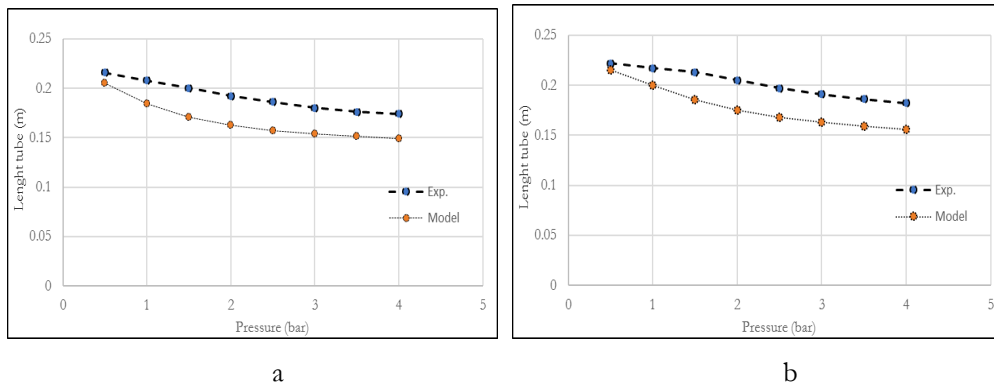
Figure 3: Model and experimental result of rig: a) force is 25N; b) force is 50N.
