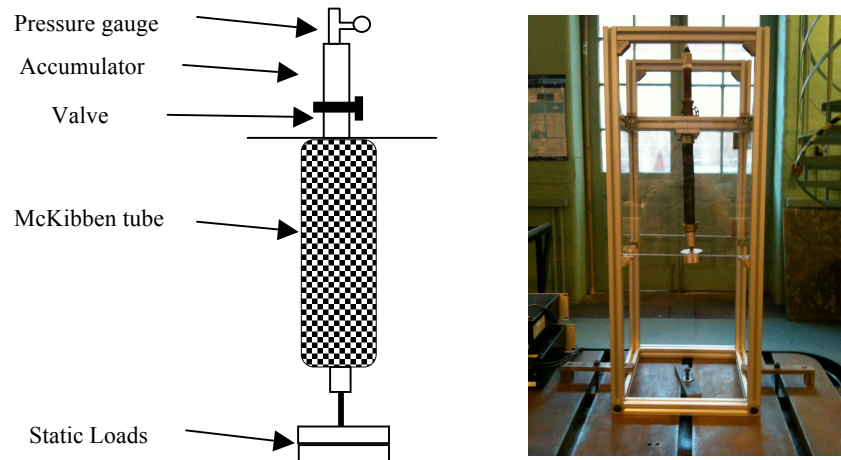
Figure 2: Test rig.
