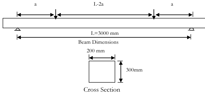
Figure 2: Details of Beam and Loading Arrangement
