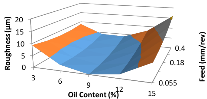
Figure 2: Relationship between roughness, oil content and cutting feed
