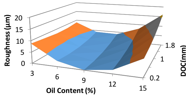
Figure 3: Relationship between roughness, oil content and depth of cutting
