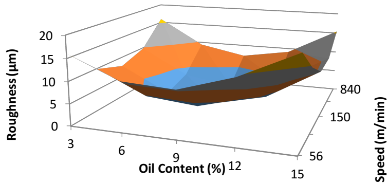
Figure 1: Relationship between roughness, oil content and cutting speed
