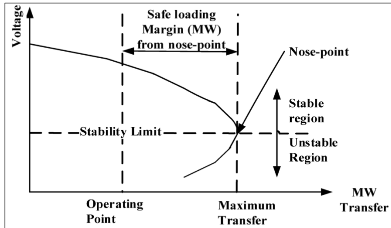
Figure 1: P-V curve and maximum loadability limit
