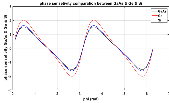
Figure 10: Comparison of phase sensitivity of (GaAs) & (Ge) & (Si) as function of \Phi . The temperature sensitivity of the Fabry-Perot's phase shift is given by:
