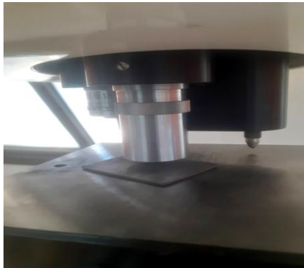
Figure1. Microhardness(Innovatest).
