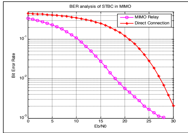
Figure 4. BER for MIMO using relay (MIMO relay) and MIMO without relay (Direct Connection).
