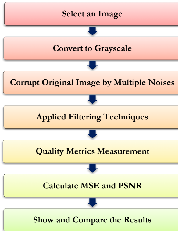
Figure 3: Methodology Structure
