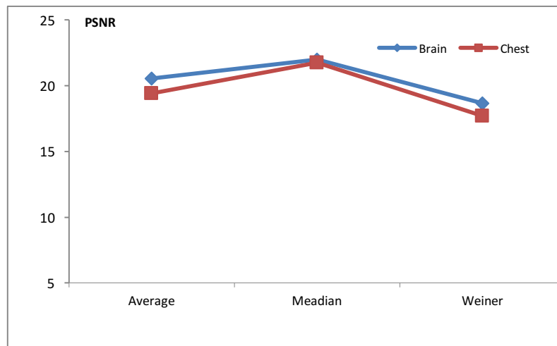
Figure 5: PSNR values
