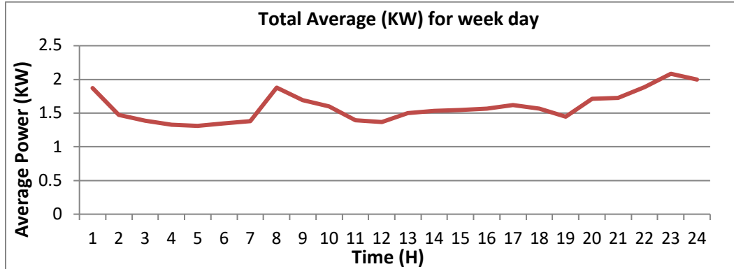
Figure (5): The average daily loads curve for all flats with two types on week days.
