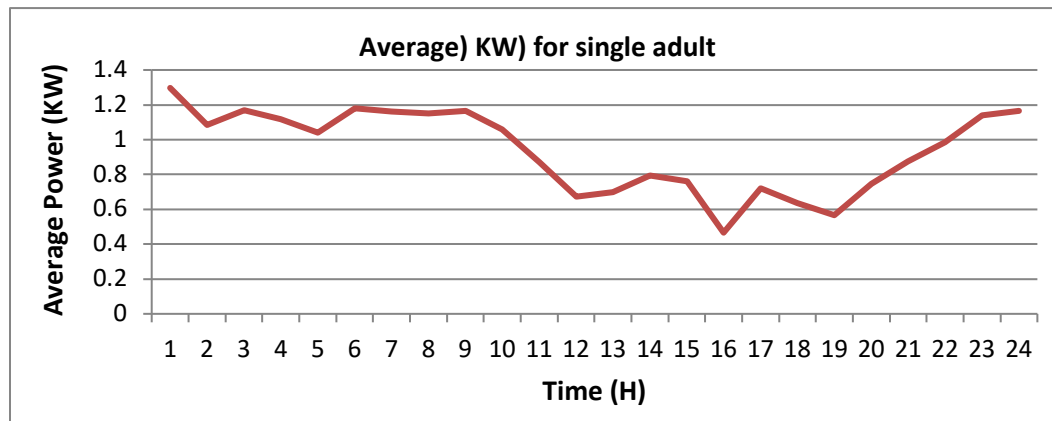
Figure (1): The average daily load curve for single adult flats during week days.
