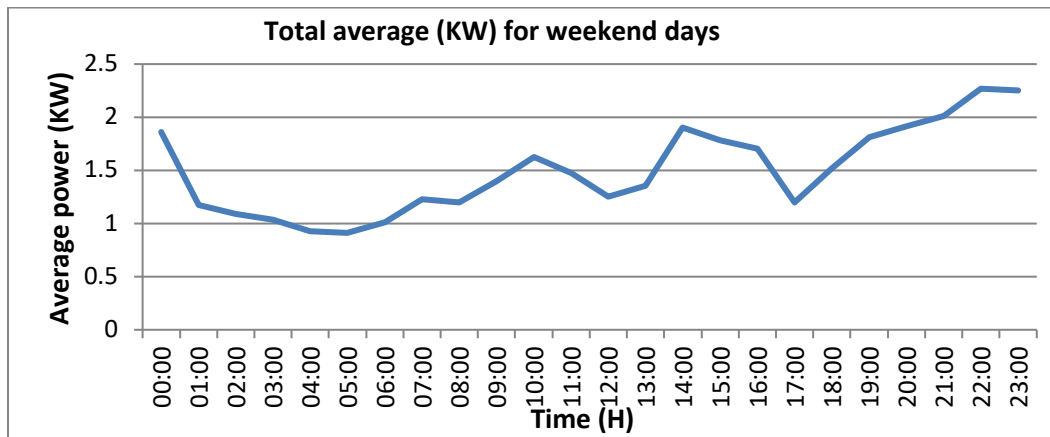
Figure (6): The average daily loads curve for all flats with two types during weekends.
