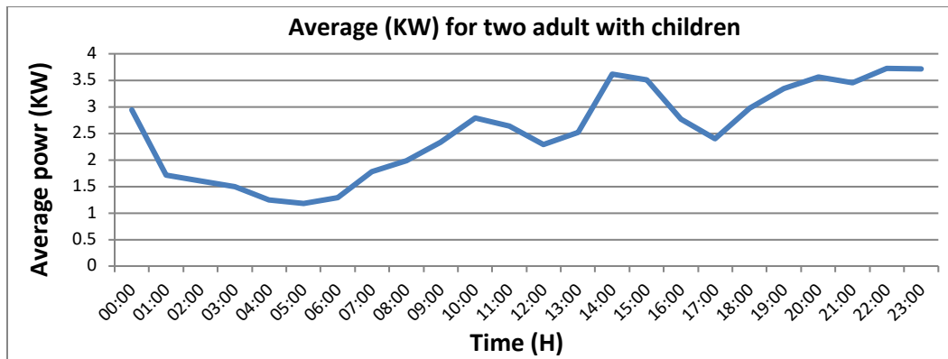
Figure (4): The average daily load curve for two adults with children during weekends.
