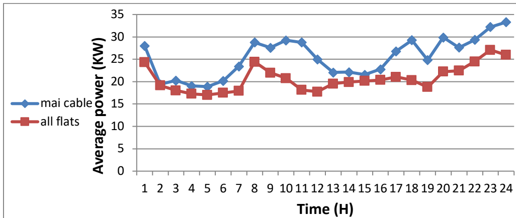
Figure (8): The average daily load curves for the main cable and all flats in building No. 2.
