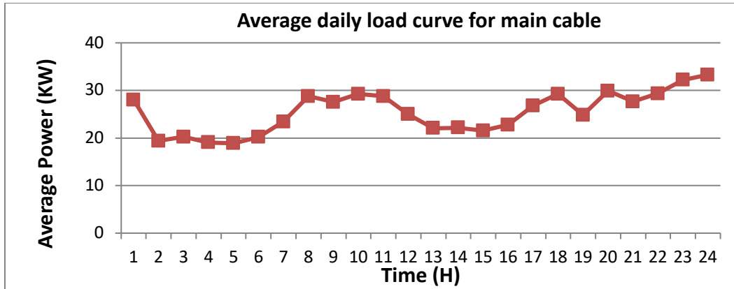
Figure (7): The average daily Power (KW) for the main distribution box during week days.
