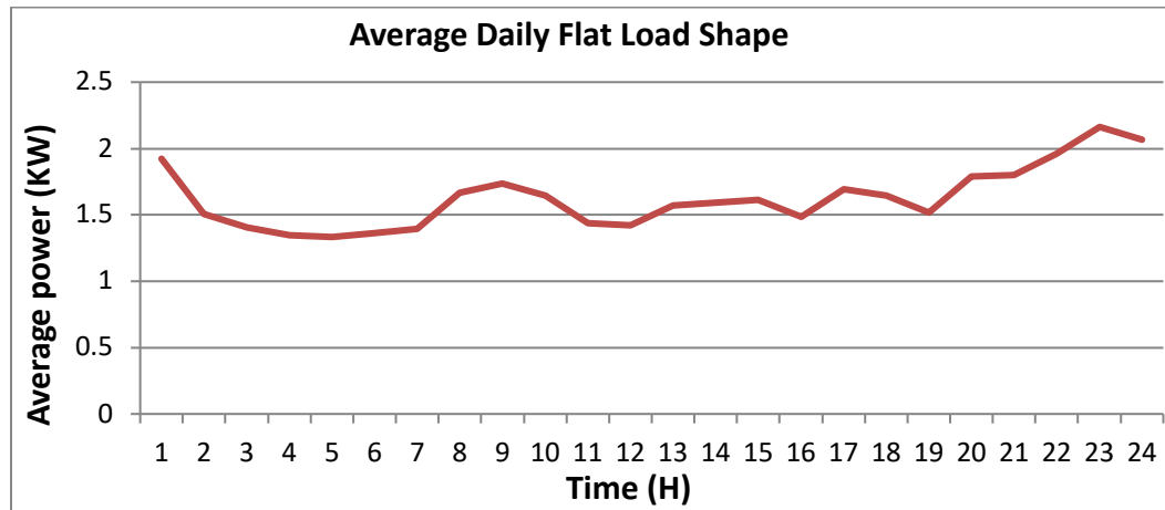
Figure (9): The average Daily Flat Load Shape.
