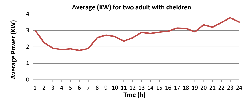
Figure (3): The average daily load curve for two adults with children during week days.
